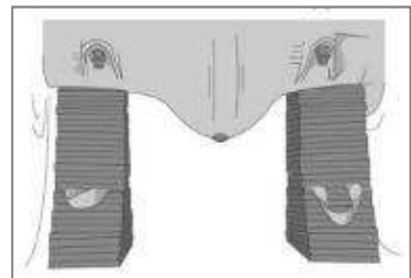
Fig. 4.6.5.2.3(1) Sleeper shoring
