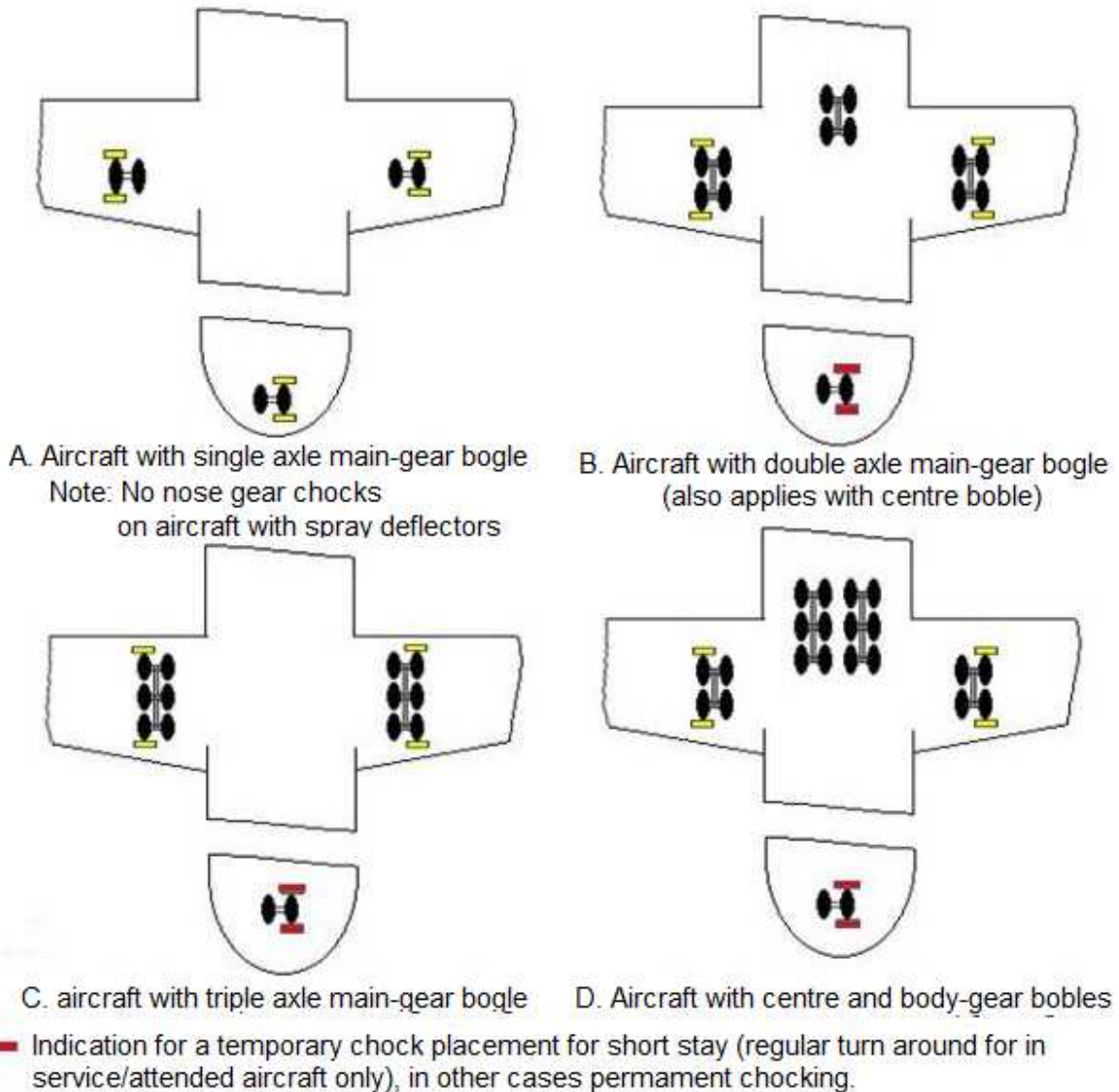
Fig. 5.6.2(1) Regular chock placement diagram
