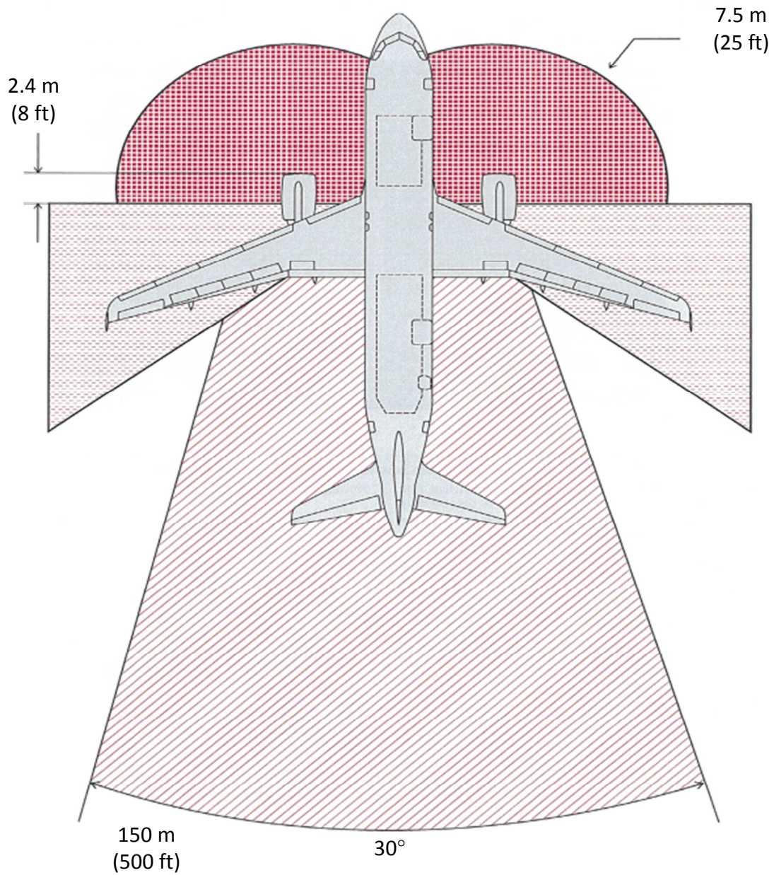
Fig. 5.1.2.2(2) Breakaway power safety area of an airplane
