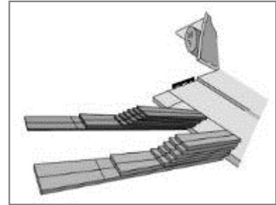
Fig. 4.6.5.2.3(1) Approach shoring
