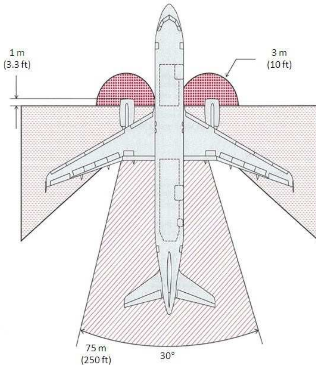
Fig 5.1.2.2(1) Idle power safety area of an airplane
