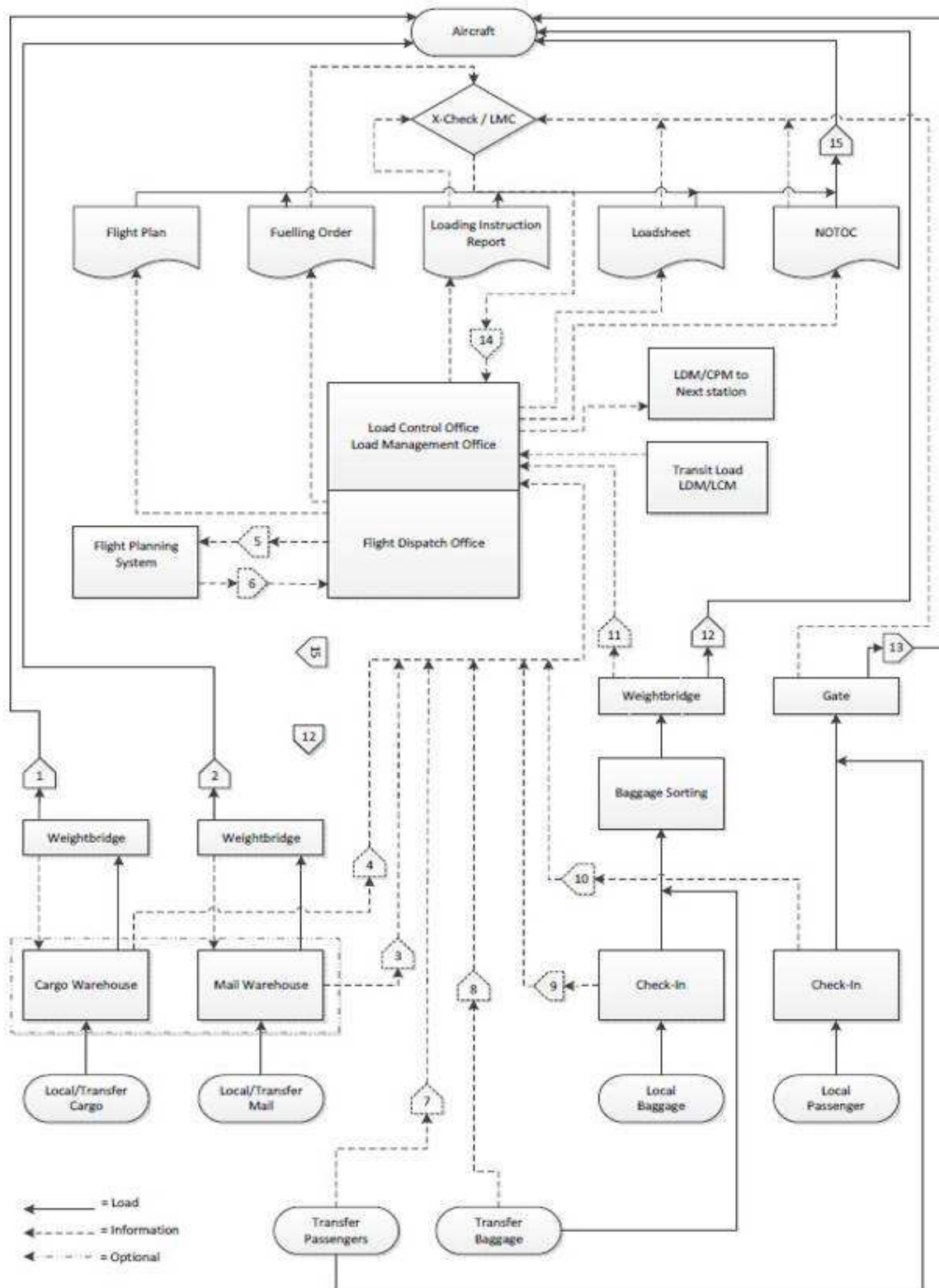
Fig. 7.3(1) Load control process flow diagram
