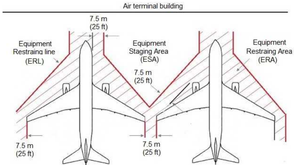
Fig. 5.1.2.3(1) Safety zone at 7,50 meters from any point of an aircraft
